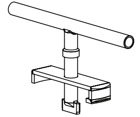
Handle Seat Removal Tool 272SW 273SW 274SW 275SW
