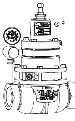
SCREWED (NPT)
