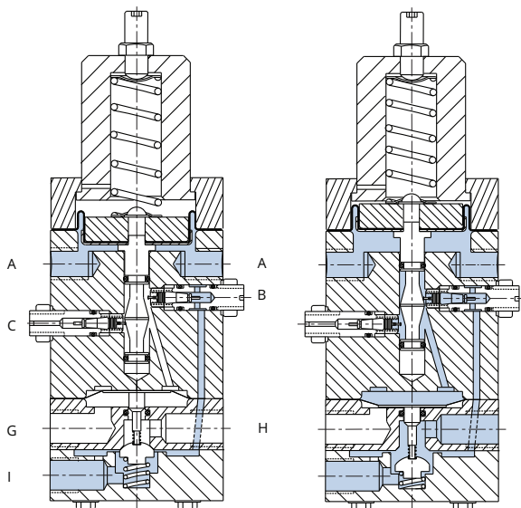
TRIP CLOSE
