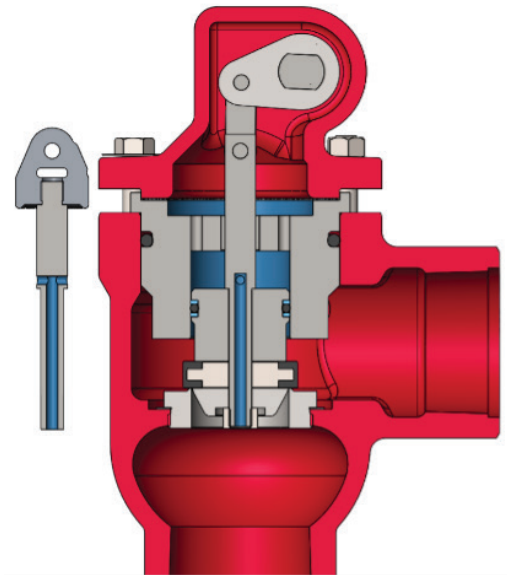
On the left is shown the old style stem with diaphragm nut attached. The new stem is shown installed in the valve.
