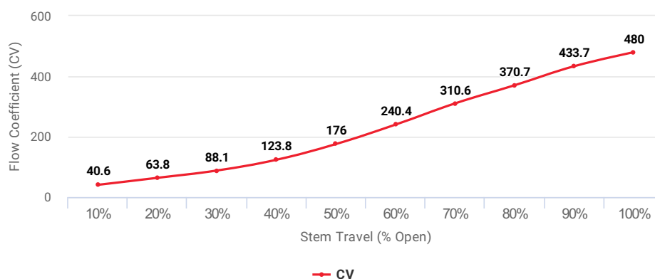
Flow Coefficient (CV) at Stem Travel (% Open) for Item: AAYS6
