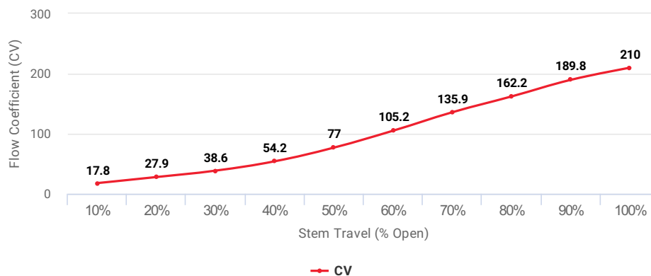
Flow Coefficient (CV) at Stem Travel (% Open) for Item: AAW
