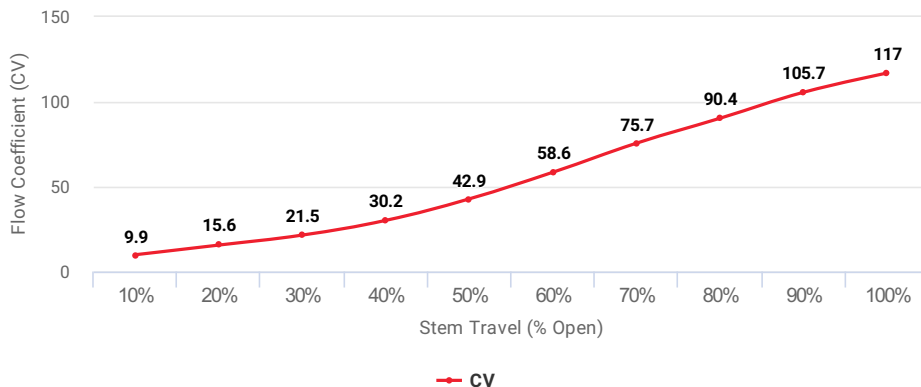
Flow Coefficient (CV) at Stem Travel (% Open) for Item: AAUV
