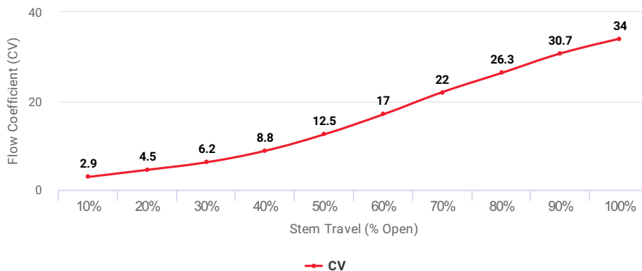
Flow Coefficient (CV) at Stem Travel (% Open) for Item: AAU5
