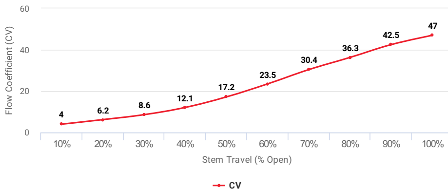
Flow Coefficient (CV) at Stem Travel (% Open) for Item: ASE
