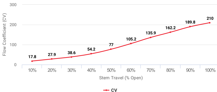
Flow Coefficient (CV) at Stem Travel (% Open) for Item: AOZD5
