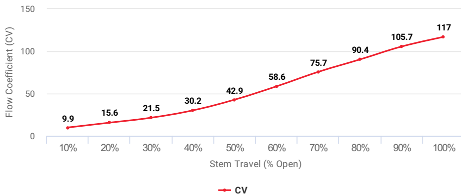
Flow Coefficient (CV) at Stem Travel (% Open) for Item: AOVD20
