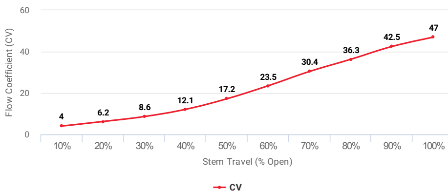
Flow Coefficient (CV) at Stem Travel (% Open) for Item: AAR
