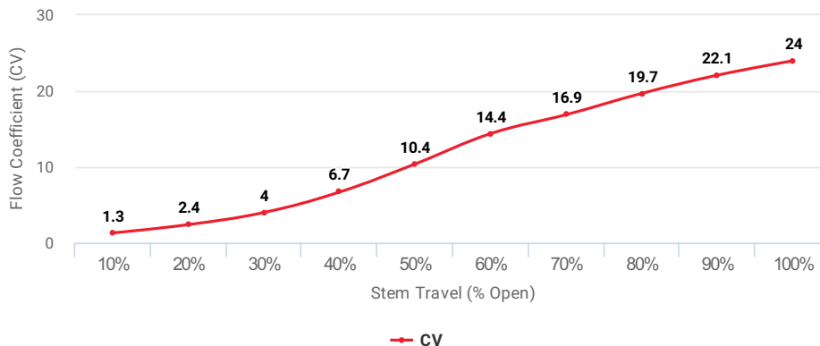
Flow Coefficient (CV) at Stem Travel (% Open) for Item: ALY4
