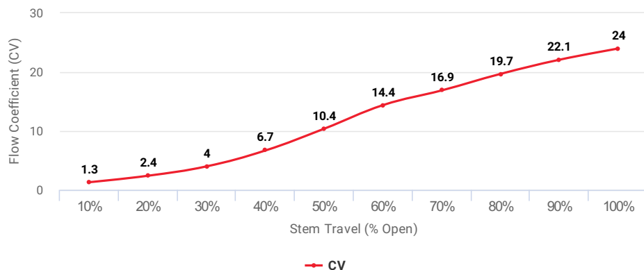
Flow Coefficient (CV) at Stem Travel (% Open) for Item: ALY12
