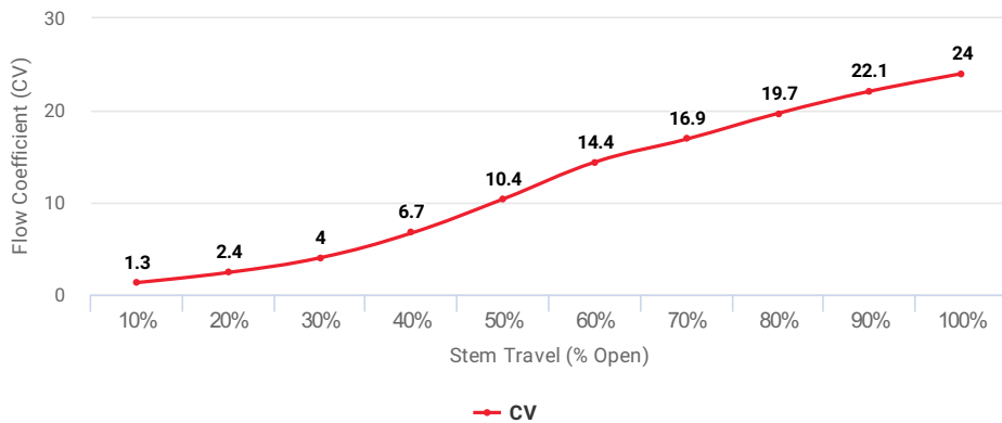
Flow Coefficient (CV) at Stem Travel (% Open) for Item: ALY1
