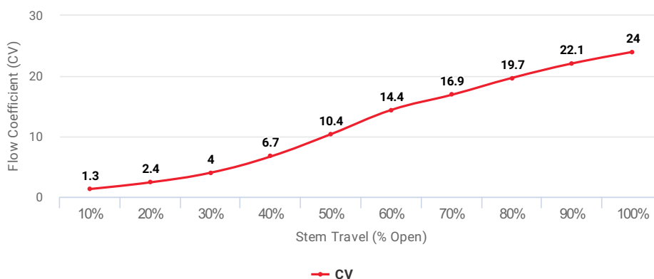
Flow Coefficient (CV) at Stem Travel (% Open) for Item: ALW6
