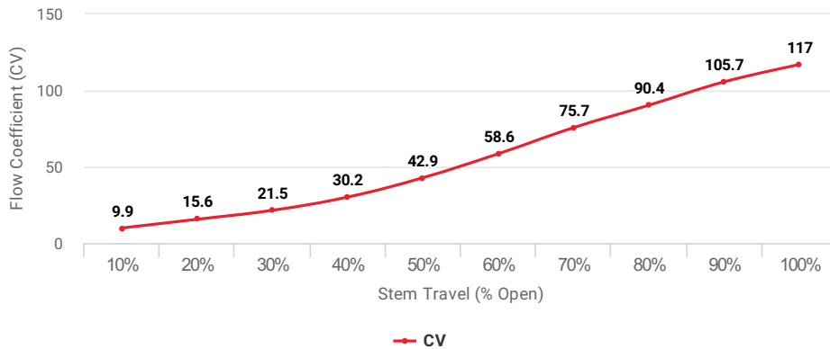
Flow Coefficient (CV) at Stem Travel (% Open) for Item: ALID
