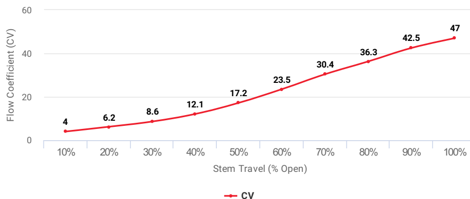
Flow Coefficient (CV) at Stem Travel (% Open) for Item: ALGD
