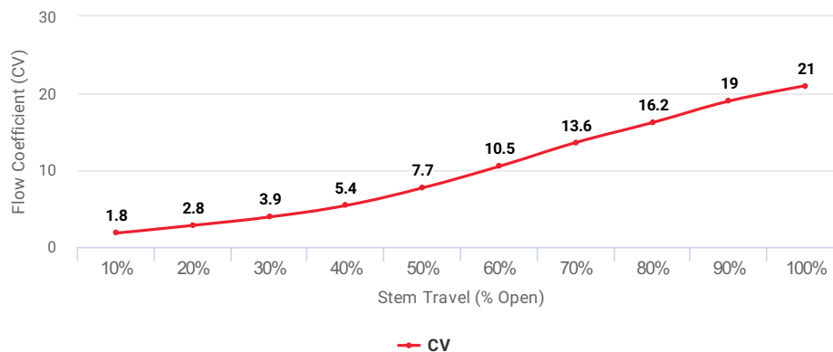
Flow Coefficient (CV) at Stem Travel (% Open) for Item: ALED5
