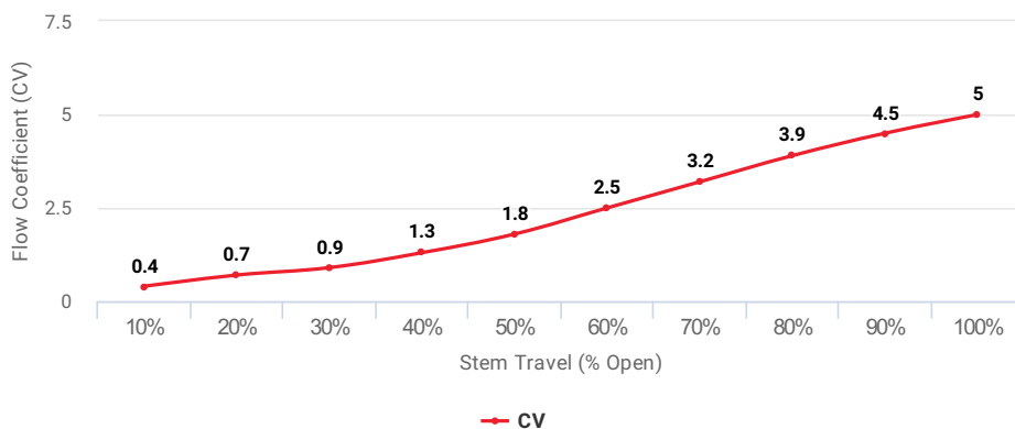
Flow Coefficient (CV) at Stem Travel (% Open) for Item: AKG5
