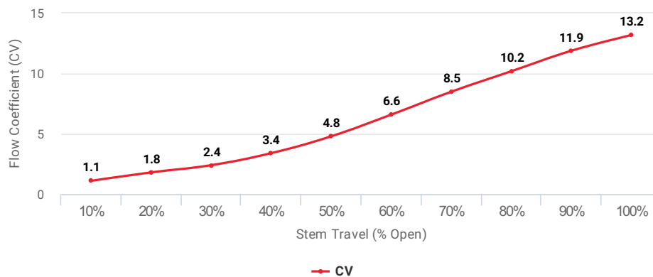
Flow Coefficient (CV) at Stem Travel (% Open) for Item: AKF
