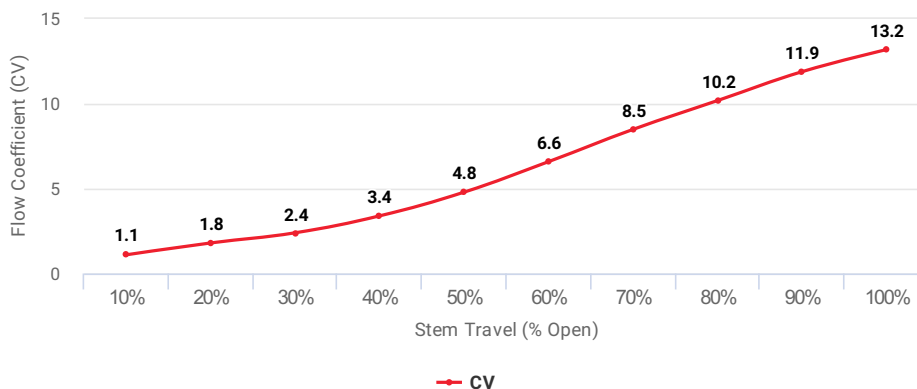
Flow Coefficient (CV) at Stem Travel (% Open) for Item: AKB
