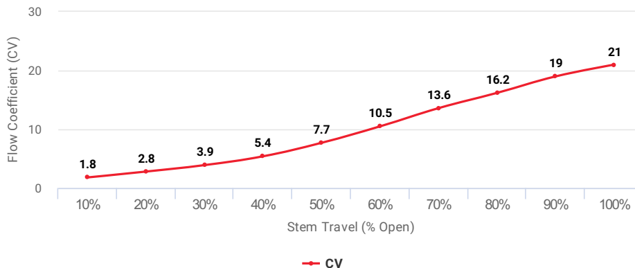
Flow Coefficient (CV) at Stem Travel (% Open) for Item: AJJ5
