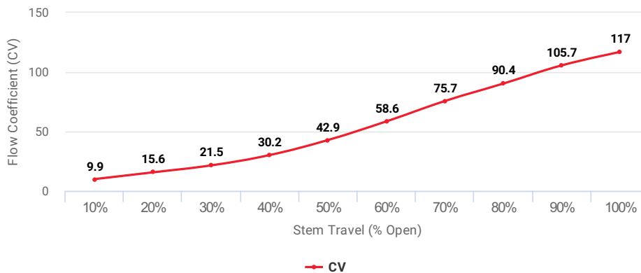
Flow Coefficient (CV) at Stem Travel (% Open) for Item: AHB20
