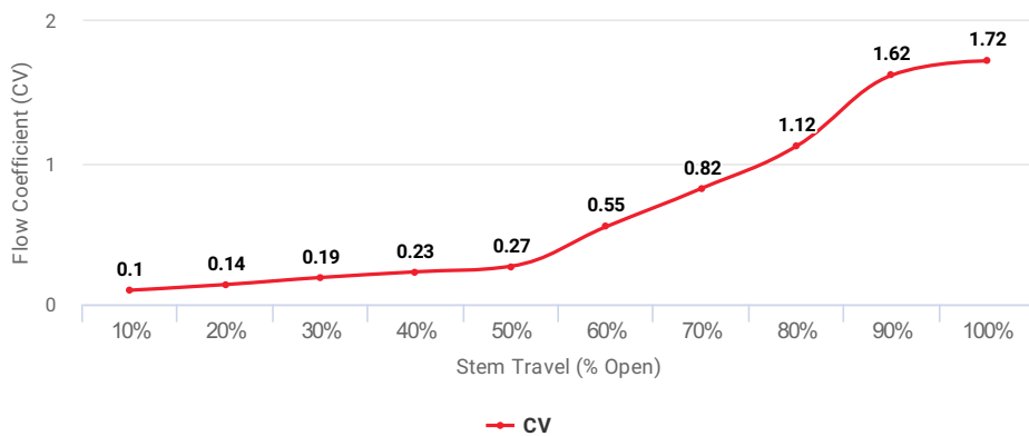
Flow Coefficient (CV) at Stem Travel (% Open) for Item: MFL
