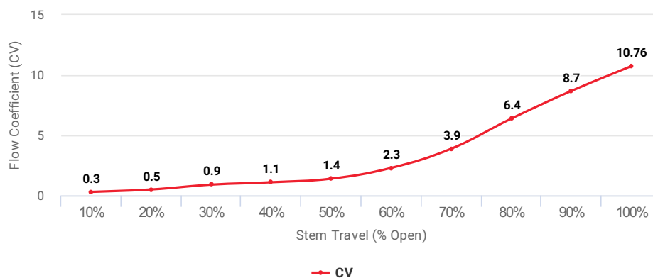
Flow Coefficient (CV) at Stem Travel (% Open) for Item: MDG
