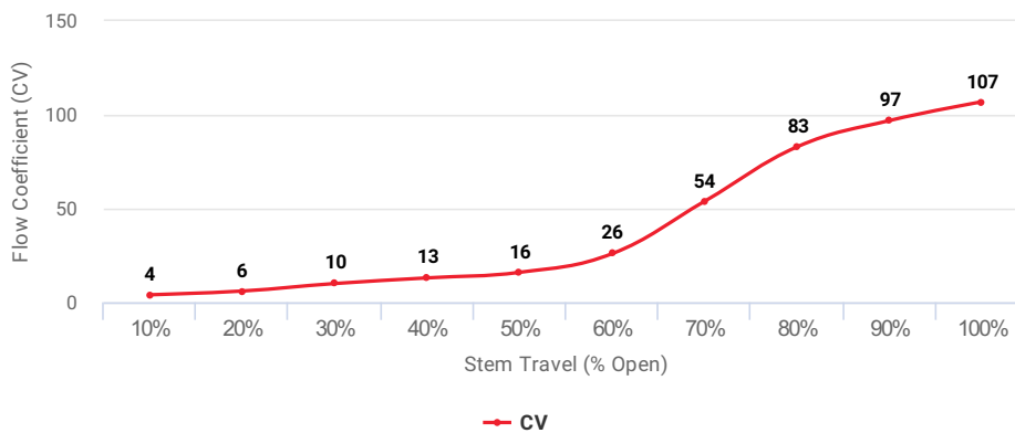
Flow Coefficient (CV) at Stem Travel (% Open) for Item: MDE
