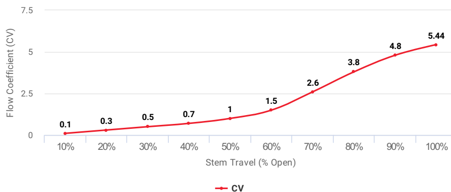
Flow Coefficient (CV) at Stem Travel (% Open) for Item: MDB
