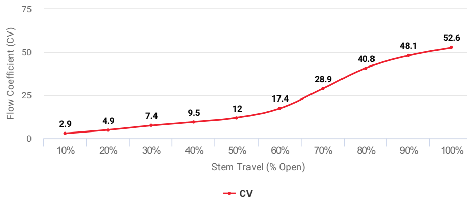
Flow Coefficient (CV) at Stem Travel (% Open) for Item: MCS
