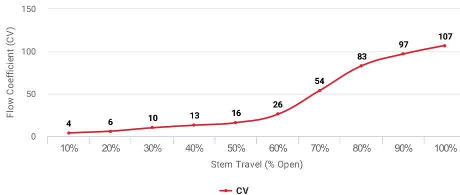
Flow Coefficient (CV) at Stem Travel (% Open) for Item: EGL
