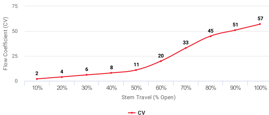
Flow Coefficient (CV) at Stem Travel (% Open) for Item: EGF
