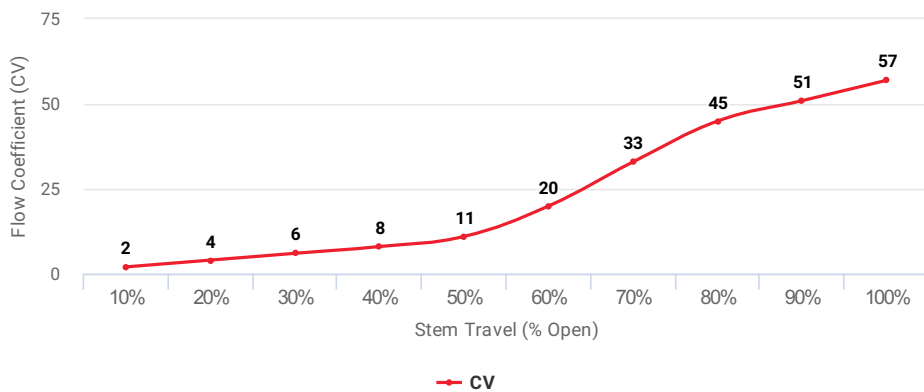
Flow Coefficient (CV) at Stem Travel (% Open) for Item: EGE
