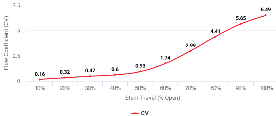
Flow Coefficient (CV) at Stem Travel (% Open) for Item: EGB
