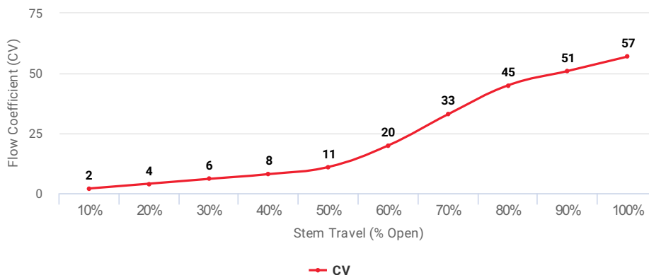
Flow Coefficient (CV) at Stem Travel (% Open) for Item: EFE
