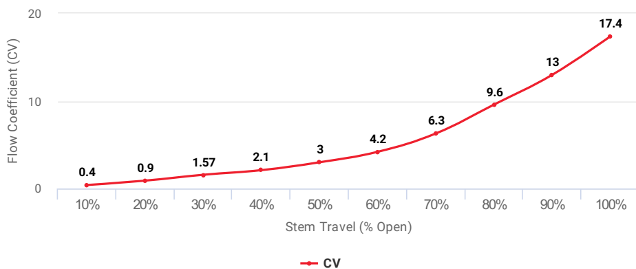
Flow Coefficient (CV) at Stem Travel (% Open) for Item: EEW
