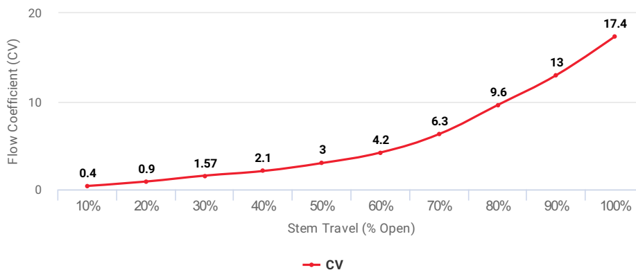
Flow Coefficient (CV) at Stem Travel (% Open) for Item: EEV
