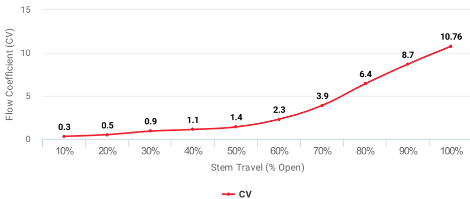
Flow Coefficient (CV) at Stem Travel (% Open) for Item: EES
