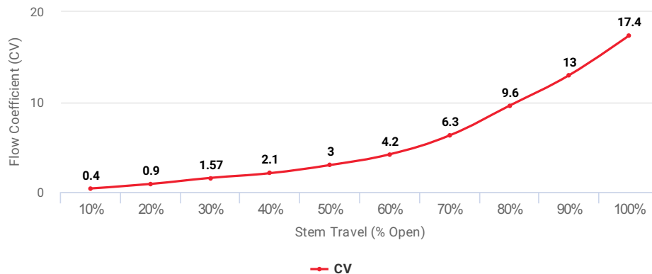
Flow Coefficient (CV) at Stem Travel (% Open) for Item: EEO
