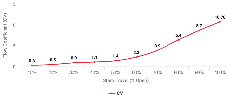
Flow Coefficient (CV) at Stem Travel (% Open) for Item: EEM
