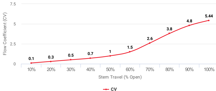
Flow Coefficient (CV) at Stem Travel (% Open) for Item: EEK
