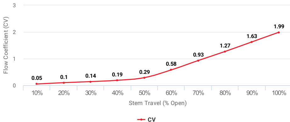
Flow Coefficient (CV) at Stem Travel (% Open) for Item: EEJ
