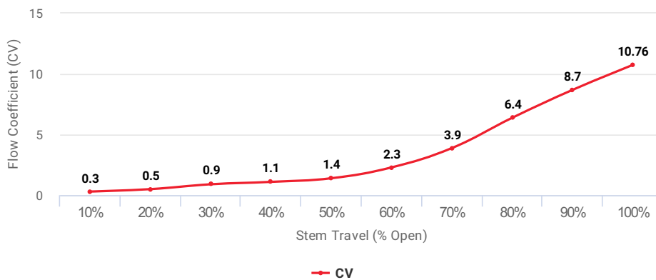
Flow Coefficient (CV) at Stem Travel (% Open) for Item: EEDV
