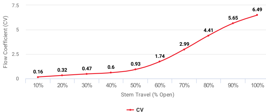
Flow Coefficient (CV) at Stem Travel (% Open) for Item: EEB
