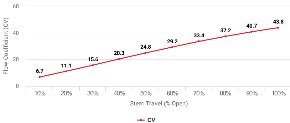
Flow Coefficient (CV) at Stem Travel (% Open) for Item: CBD
