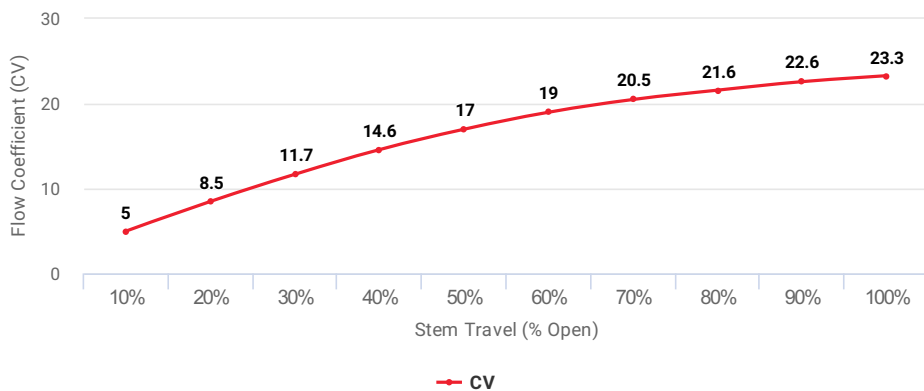
Flow Coefficient (CV) at Stem Travel (% Open) for Item: CAQ
