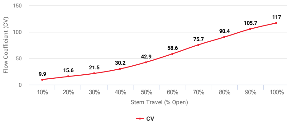
Flow Coefficient (CV) at Stem Travel (% Open) for Item: AFC20
