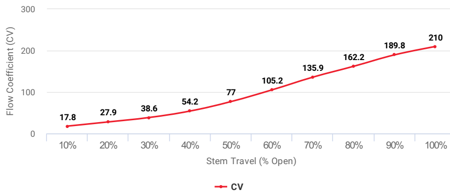
Flow Coefficient (CV) at Stem Travel (% Open) for Item: ADB
