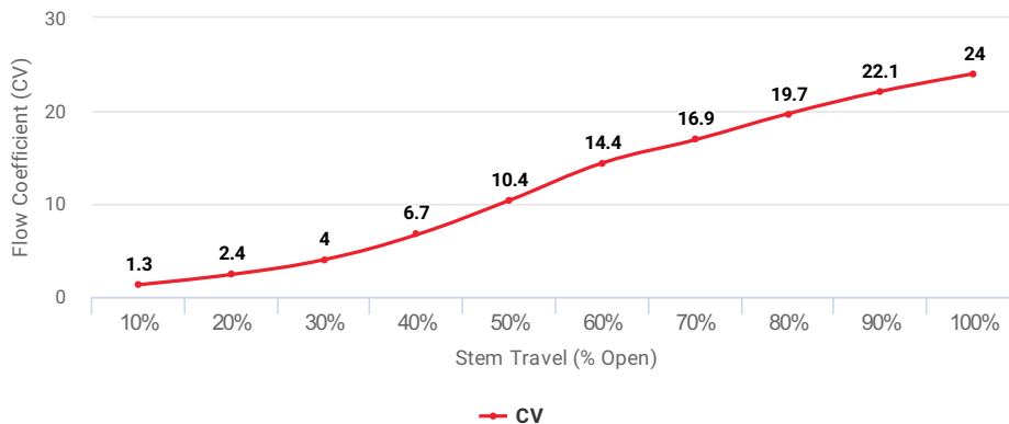
Flow Coefficient (CV) at Stem Travel (% Open) for Item: EUD3
