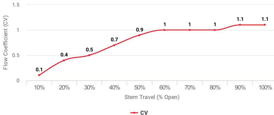
Flow Coefficient (CV) at Stem Travel (% Open) for Item: EHH
