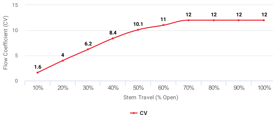
Flow Coefficient (CV) at Stem Travel (% Open) for Item: ECOPC
